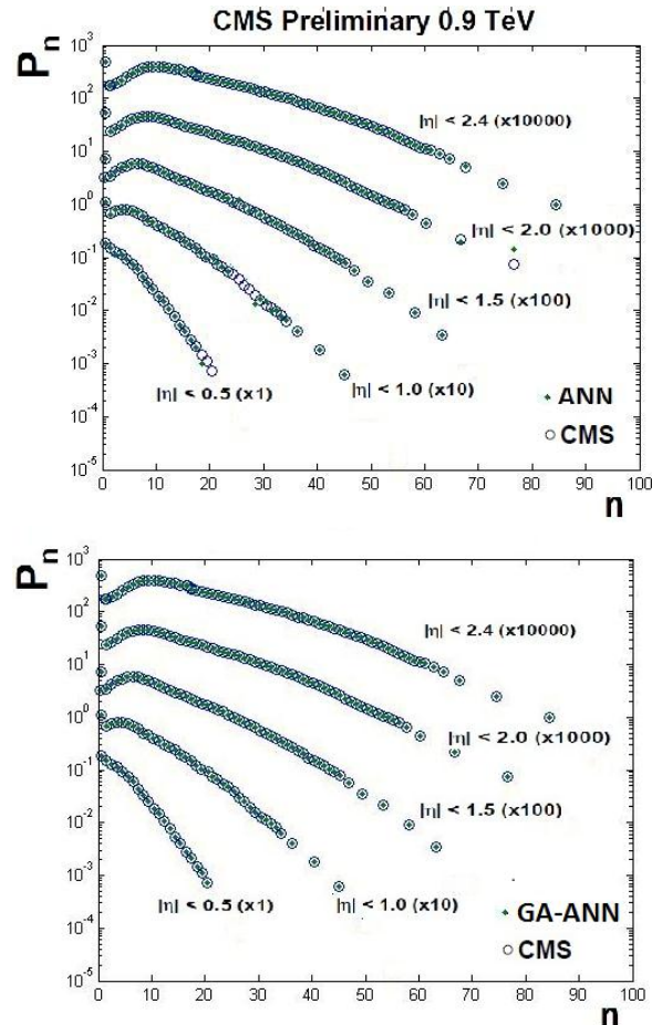
Figure 5: ANN and GA-ANN simulation results for charge particle Multiplicity distribution of shower p-p at \sqrt{s} = 0.9 TeV
