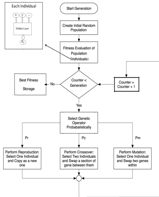
Figure 3: Overview of GA-ANN hybrid model
