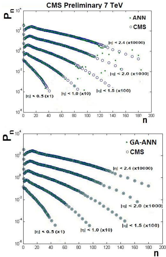
Figure 7: ANN and GA-ANN simulation results for charge particle Multiplicity distribution of shower p-p at \sqrt{s} = 7 TeV
